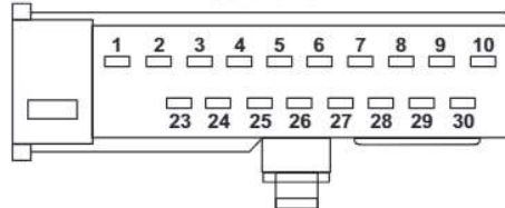
TCM "C1" Connector
