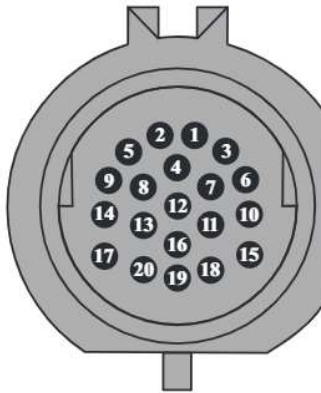
View Looking Into The External Transaxle Harness Connector Number "T20h"
