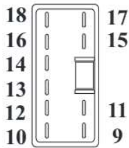
Internal Transaxle Harness "Male" Coupler Connector Number "H2-04"
