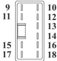
View Looking Into The Internal Transaxle Harness "Male" Coupler Connector Number "T10"
