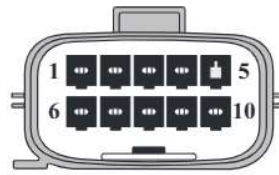
View Looking Into JB156 Connector
