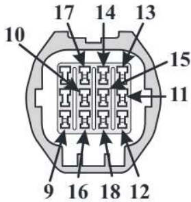
External Transaxle Harness Connector Number "H2-03"
