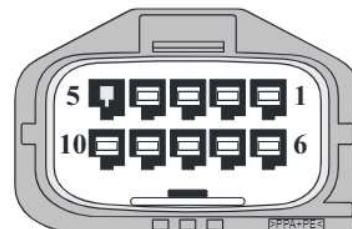
View Looking Into Vehicle Harness Connector JB156
