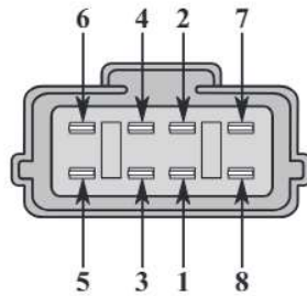
External Transaxle Connector Number "H1-05"
