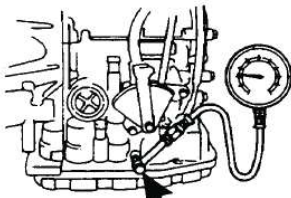
LINE PRESSURE TAP
