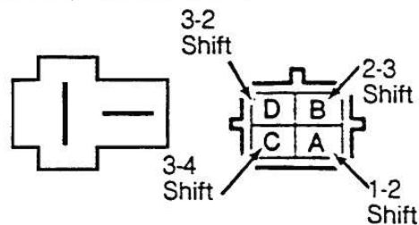
LOCKUP SOLENOID CONNECTOR
