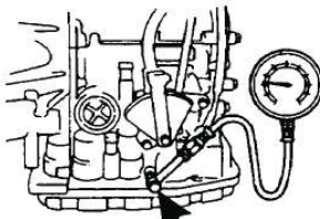
LINE PRESSURE TAP
