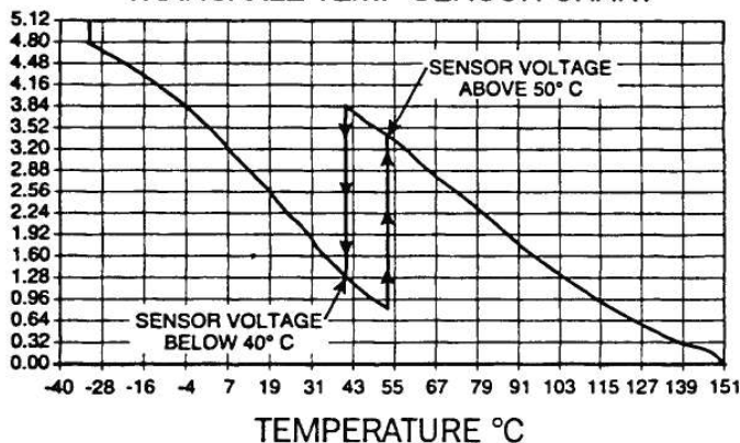
TRANSAXLE TEMP SENSOR CHART
