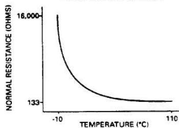
TEMPERATURE SENSOR
