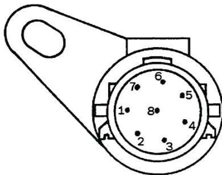
CASE CONNECTOR
